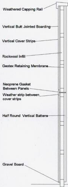
SECTION THROUGH POST
